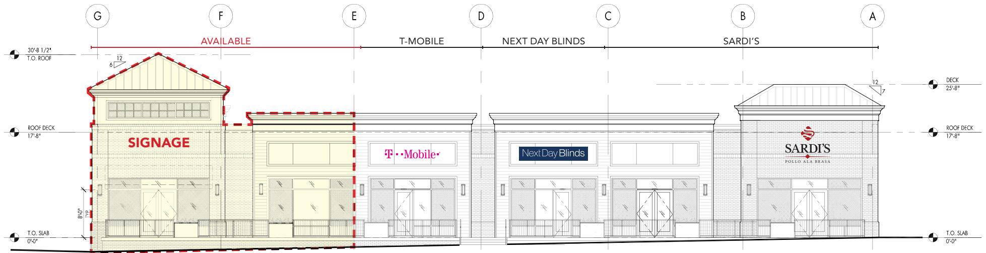
3 NORTH ELEVATION
